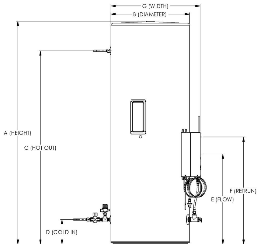
Figure 5-2 Tank and Pump Module
