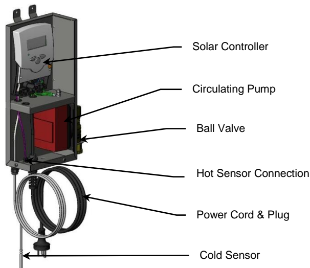
Figure 8-2 PM-600 General Arrangement
