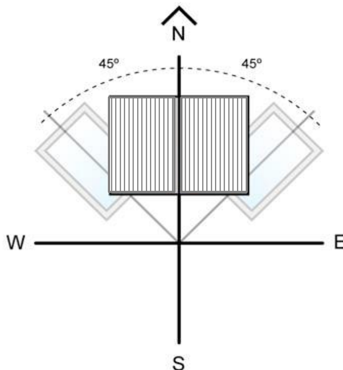
Figure 4-1 Collector orientation
